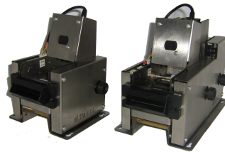
Imported motorized barcode ticket acceptor from el.tr.a.s.r.l that provides reliable and speedy ticket handling.
