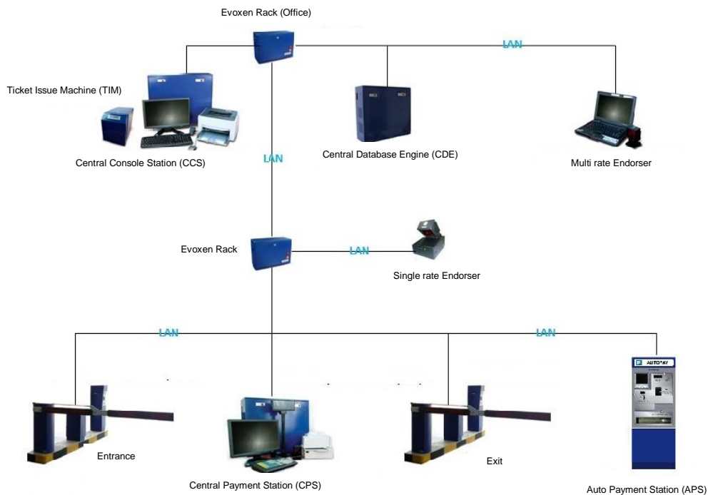
Logical Layout diagram for Central Payment Station
