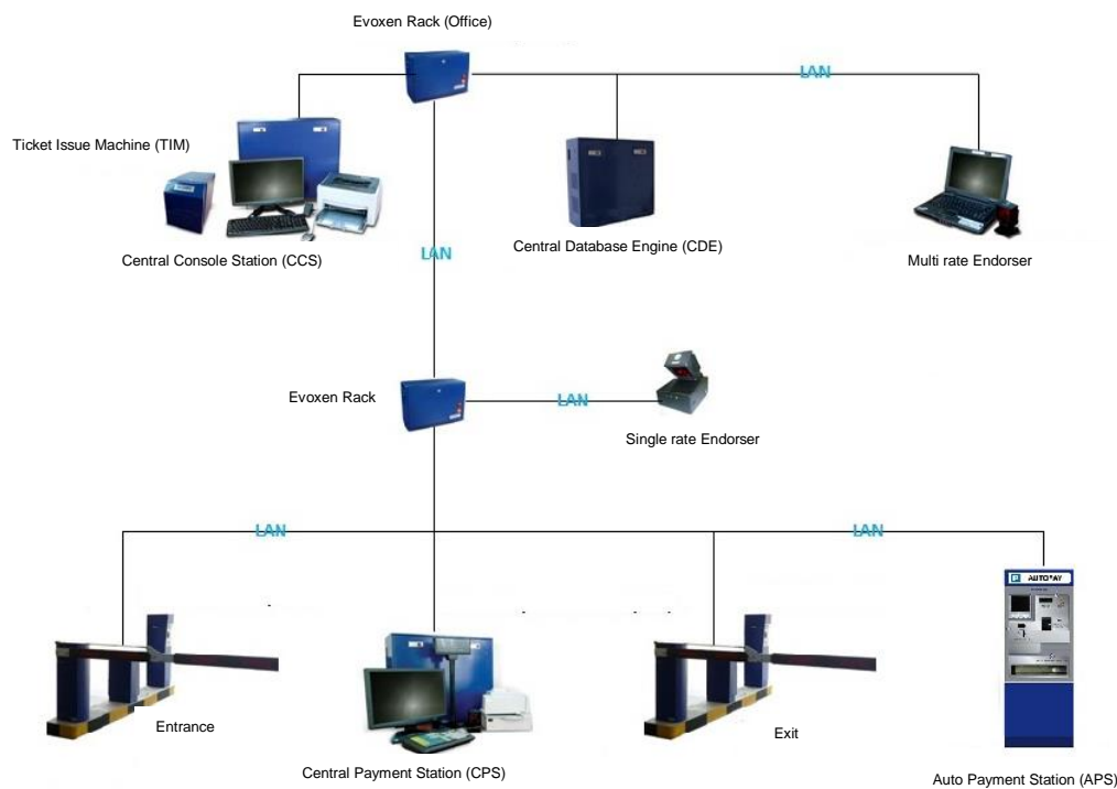
Logical Layout diagram for Central Console Station
